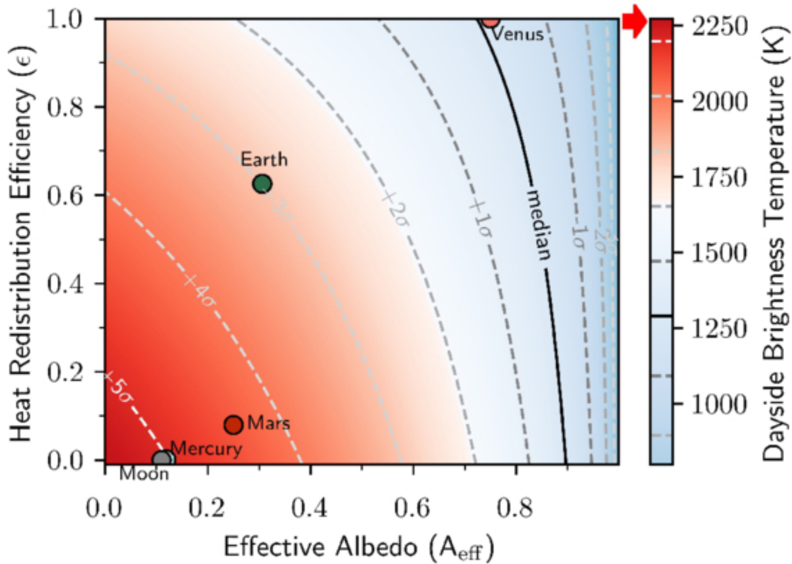
Figure 2. from Brandon Park Coy et al 2026 Astrophys. J. Lett. 1005 doi:10.3847/2041-8213/ae7f23 https://dx.doi.org/10.3847/2041-8213/ae7f23 © 2026. The Author(s). Published by the American Astronomical Society.
