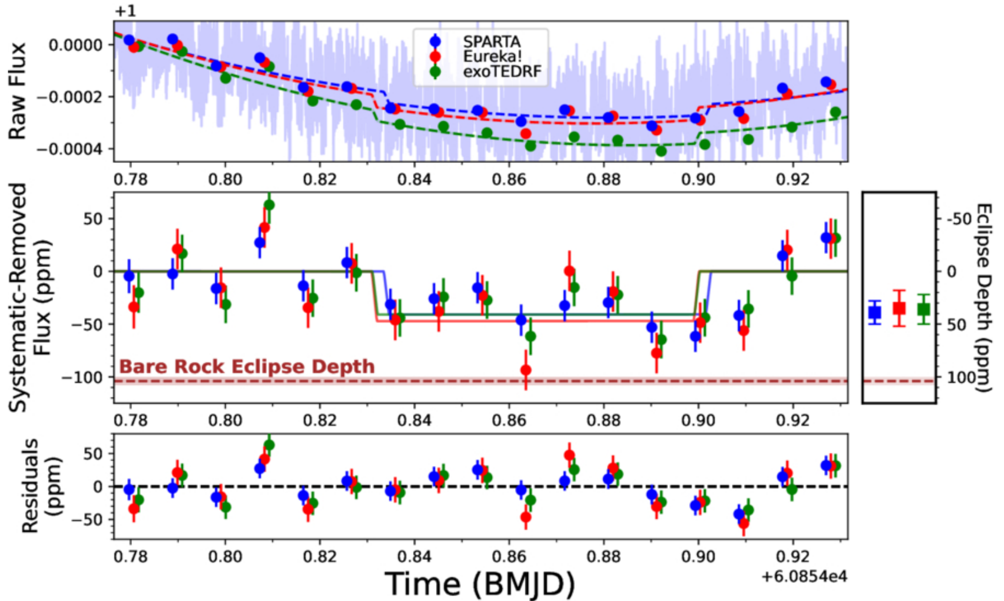
Figure 1. from Brandon Park Coy et al 2026 Astrophys. J. Lett. 1005 doi:10.3847/2041-8213/ae7f23 https://dx.doi.org/10.3847/2041-8213/ae7f23 © 2026. The Author(s). Published by the American Astronomical Society.
