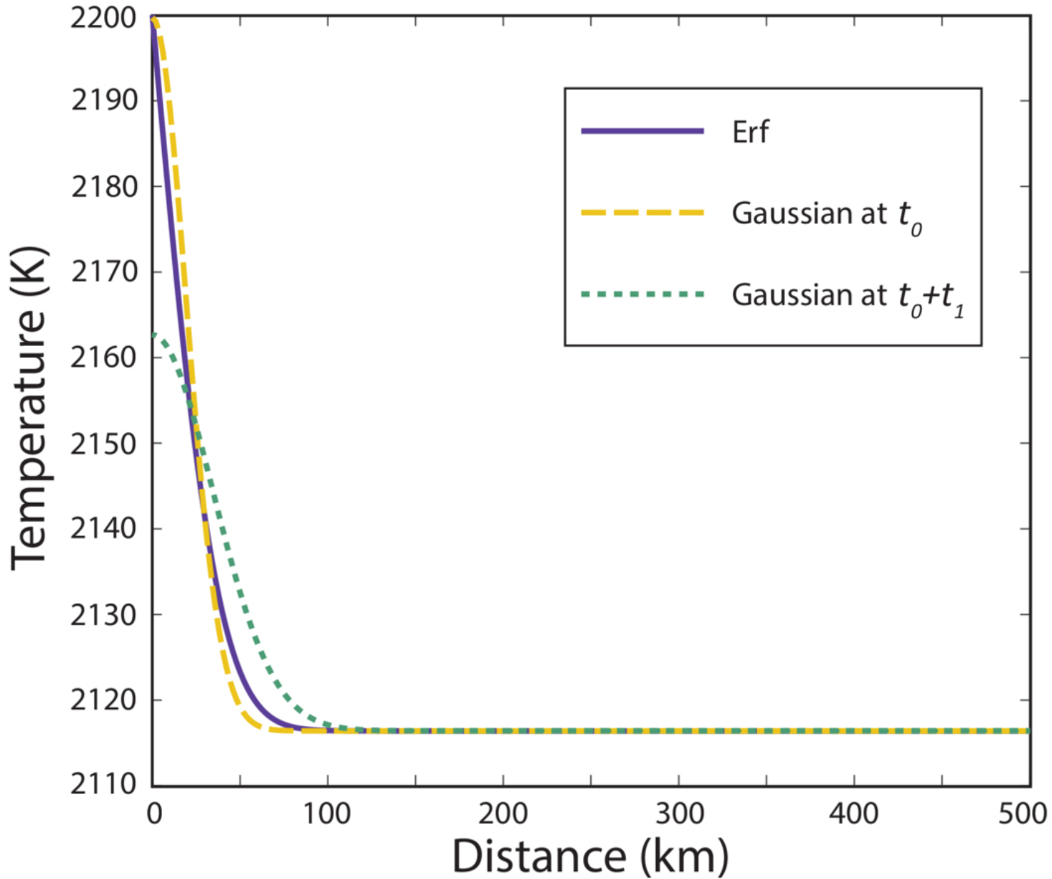
Figure 5. from Antonio Manjón-Cabeza Córdoba et al 2026 Astrophys. J. Lett. 1005 doi:10.3847/2041-8213/ae7e8b https://dx.doi.org/10.3847/2041-8213/ae7e8b © 2026. The Author(s). Published by the American Astronomical Society.
