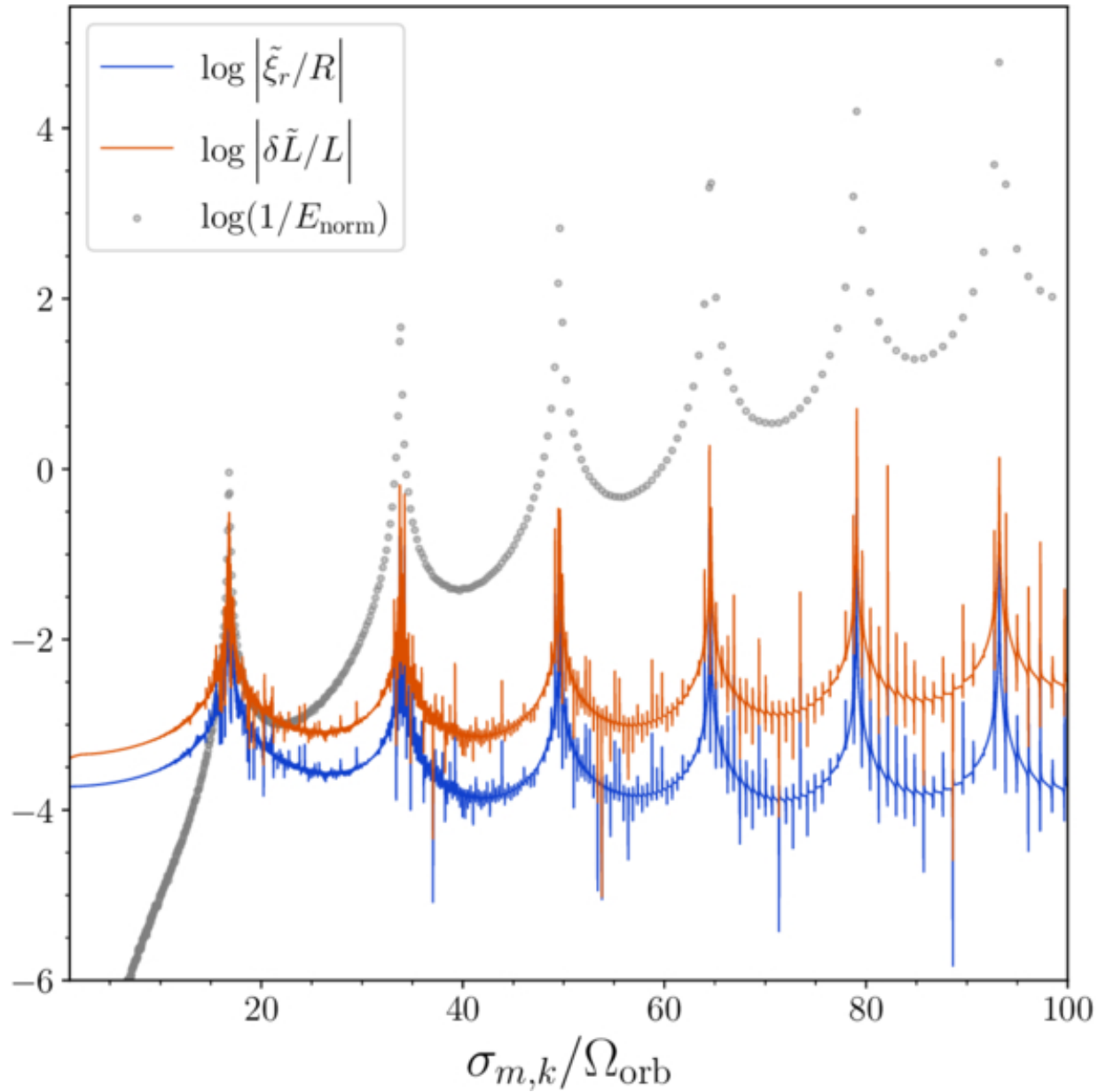
Figure 3. from Ritvik Sai Narayan et al 2026 Astrophys. J. Lett. 1005 doi:10.3847/2041-8213/ae7e89 https://dx.doi.org/10.3847/2041-8213/ae7e89 © 2026. The Author(s). Published by the American Astronomical Society.
