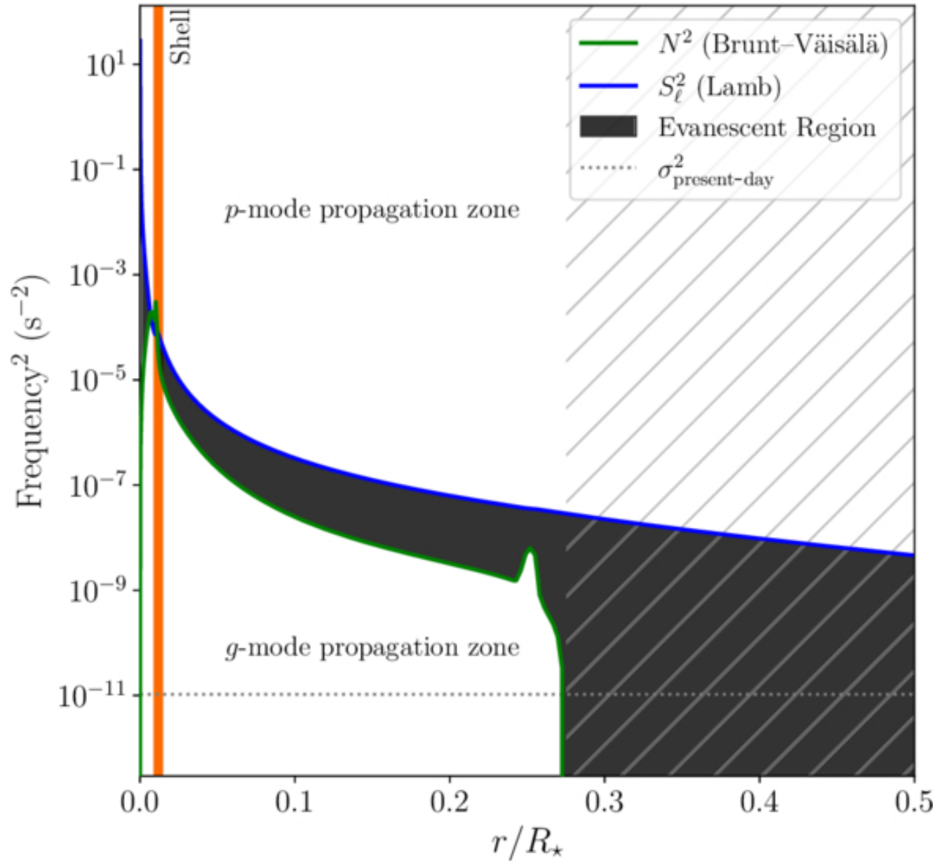
Figure 2. from Ritvik Sai Narayan et al 2026 Astrophys. J. Lett. 1005 doi:10.3847/2041-8213/ae7e89 https://dx.doi.org/10.3847/2041-8213/ae7e89 © 2026. The Author(s). Published by the American Astronomical Society.
