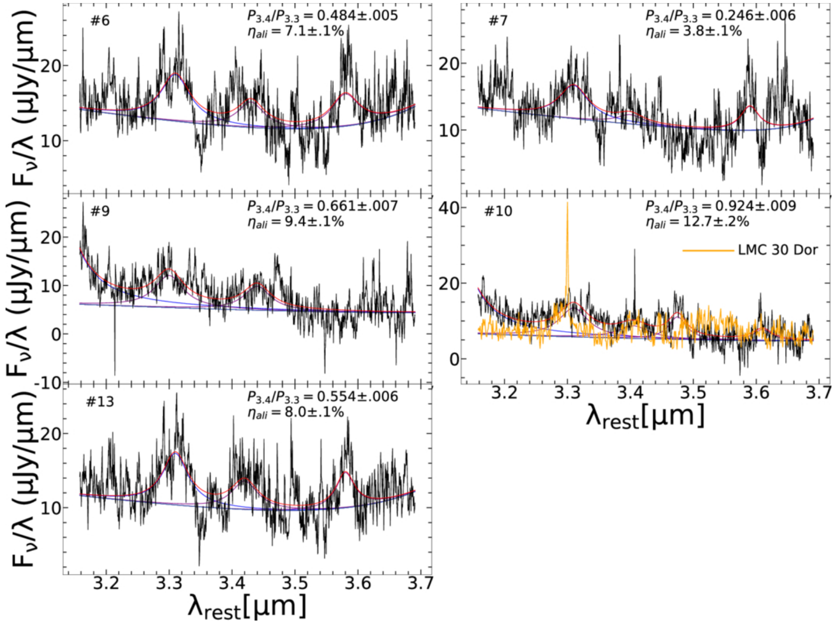
Figure 4. from C. E. Mentzer et al 2026 Astrophys. J. Lett. 1005 doi:10.3847/2041-8213/ae7e86 https://dx.doi.org/10.3847/2041-8213/ae7e86 © 2026. The Author(s). Published by the American Astronomical Society.
