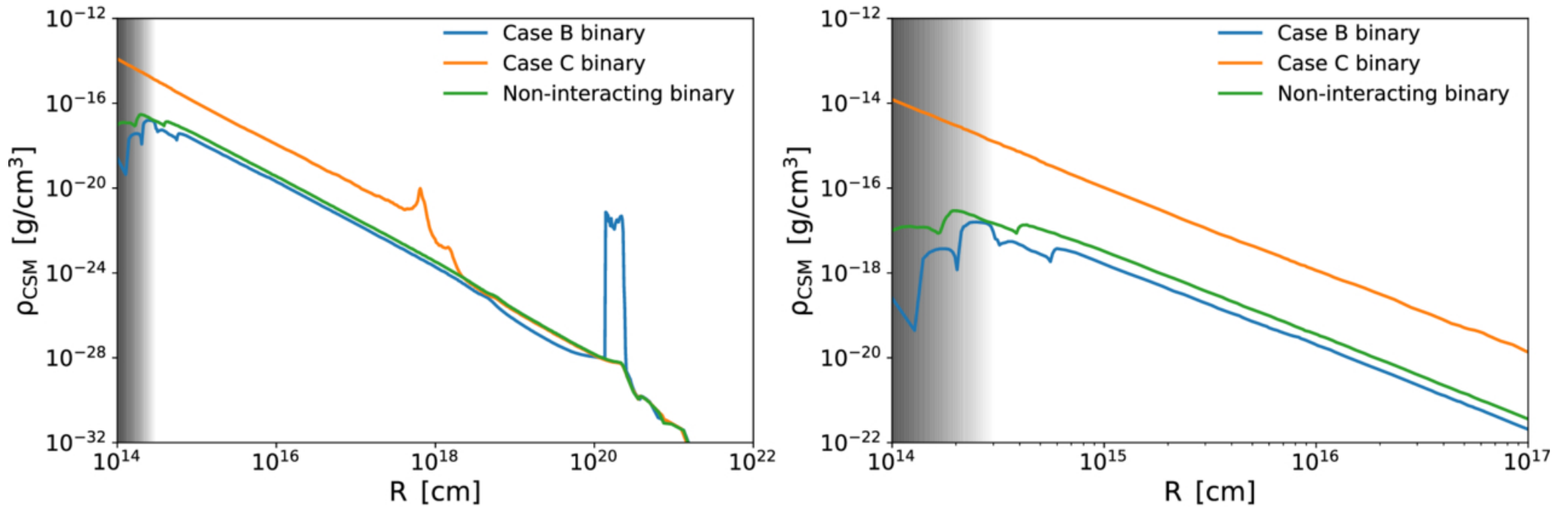
Figure 4. from Sung-Han Tsai et al 2026 Astrophys. J. Lett. 1005 doi:10.3847/2041-8213/ae7e84 https://dx.doi.org/10.3847/2041-8213/ae7e84 © 2026. The Author(s). Published by the American Astronomical Society.
