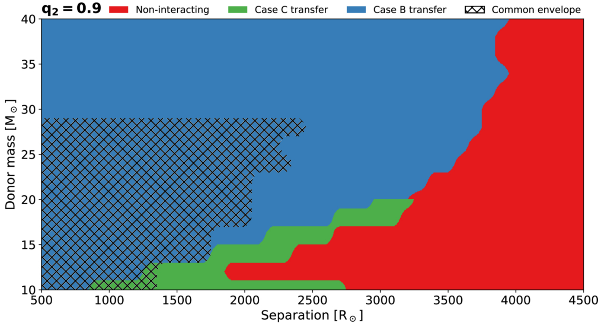
Figure 2. from Sung-Han Tsai et al 2026 Astrophys. J. Lett. 1005 doi:10.3847/2041-8213/ae7e84 https://dx.doi.org/10.3847/2041-8213/ae7e84 © 2026. The Author(s). Published by the American Astronomical Society.
