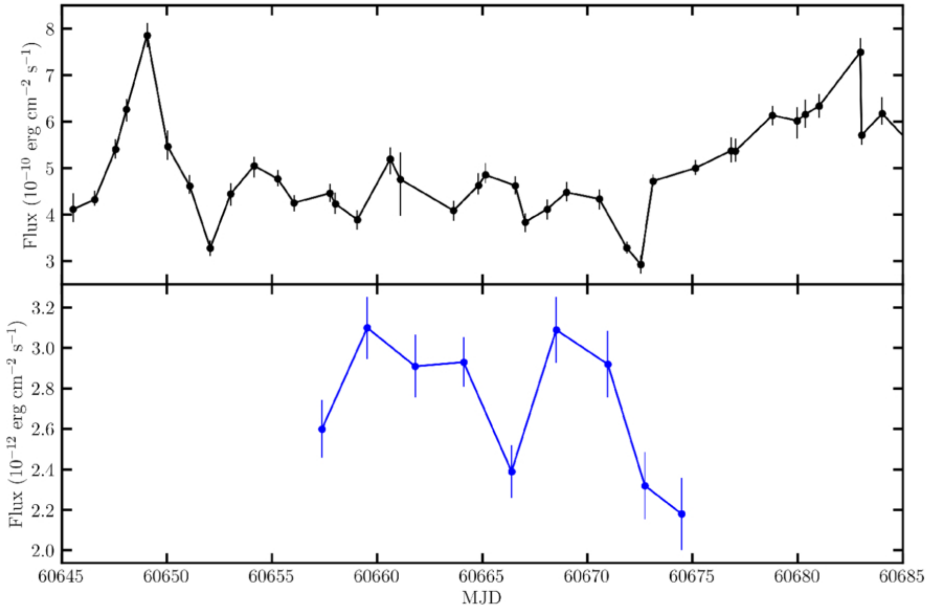
Figure 4. from Jon M. Miller et al 2026 Astrophys. J. Lett. 1005 doi:10.3847/2041-8213/ae7e82 https://dx.doi.org/10.3847/2041-8213/ae7e82 © 2026. The Author(s). Published by the American Astronomical Society.
