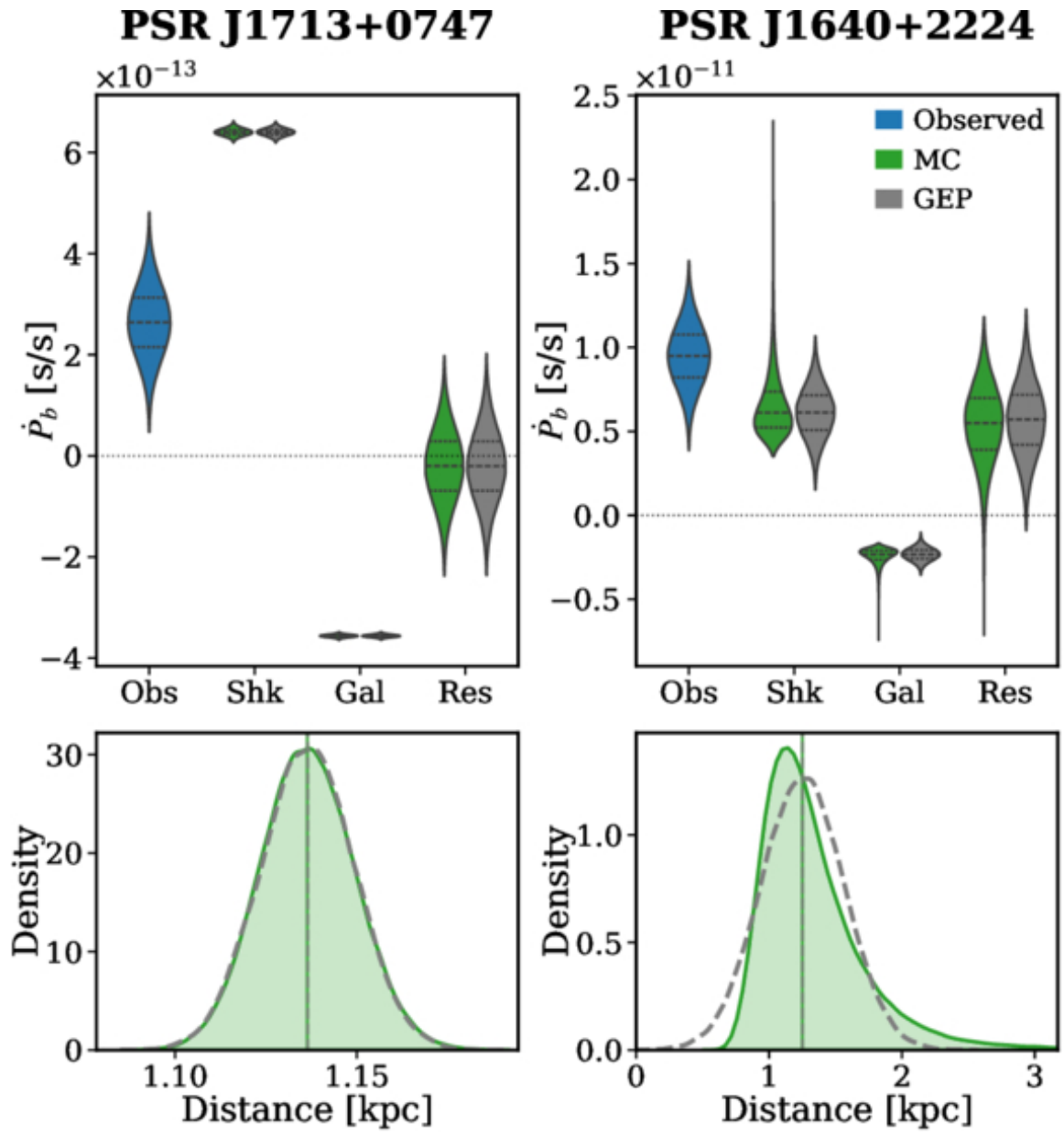
Figure 2. from Zheng-Long Wang et al 2026 Astrophys. J. Lett. 1005 doi:10.3847/2041-8213/ae7de6 https://dx.doi.org/10.3847/2041-8213/ae7de6 © 2026. The Author(s). Published by the American Astronomical Society.
