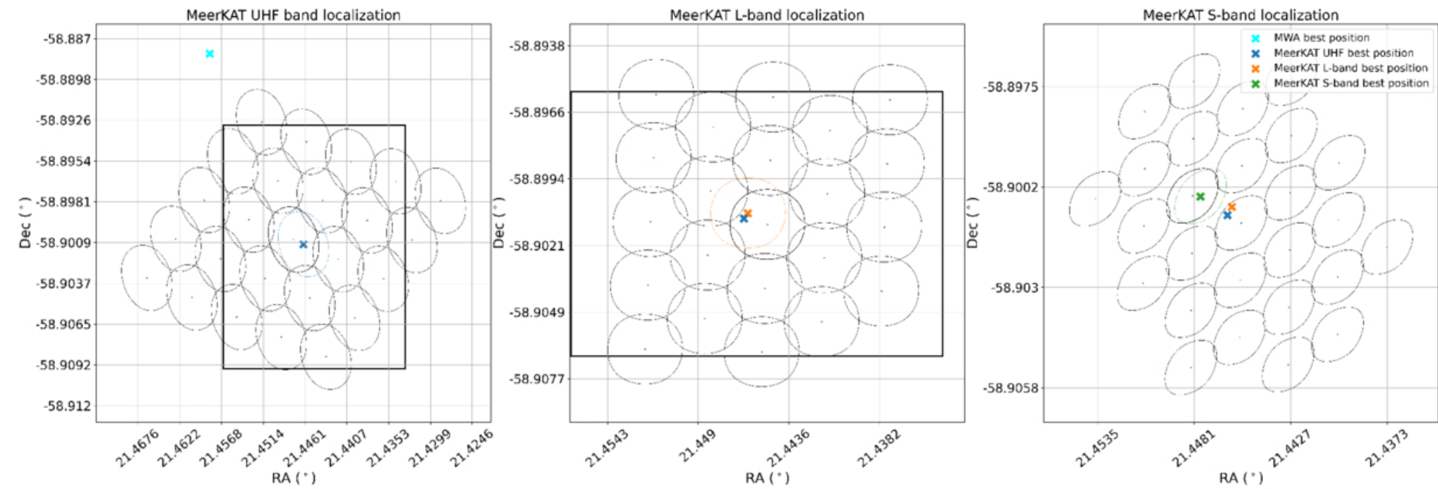
Figure 6. from Chia Min Tan et al 2026 Astrophys. J. Lett. 1006 doi:10.3847/2041-8213/ae7de5 https://dx.doi.org/10.3847/2041-8213/ae7de5 © 2026. The Author(s). Published by the American Astronomical Society.
