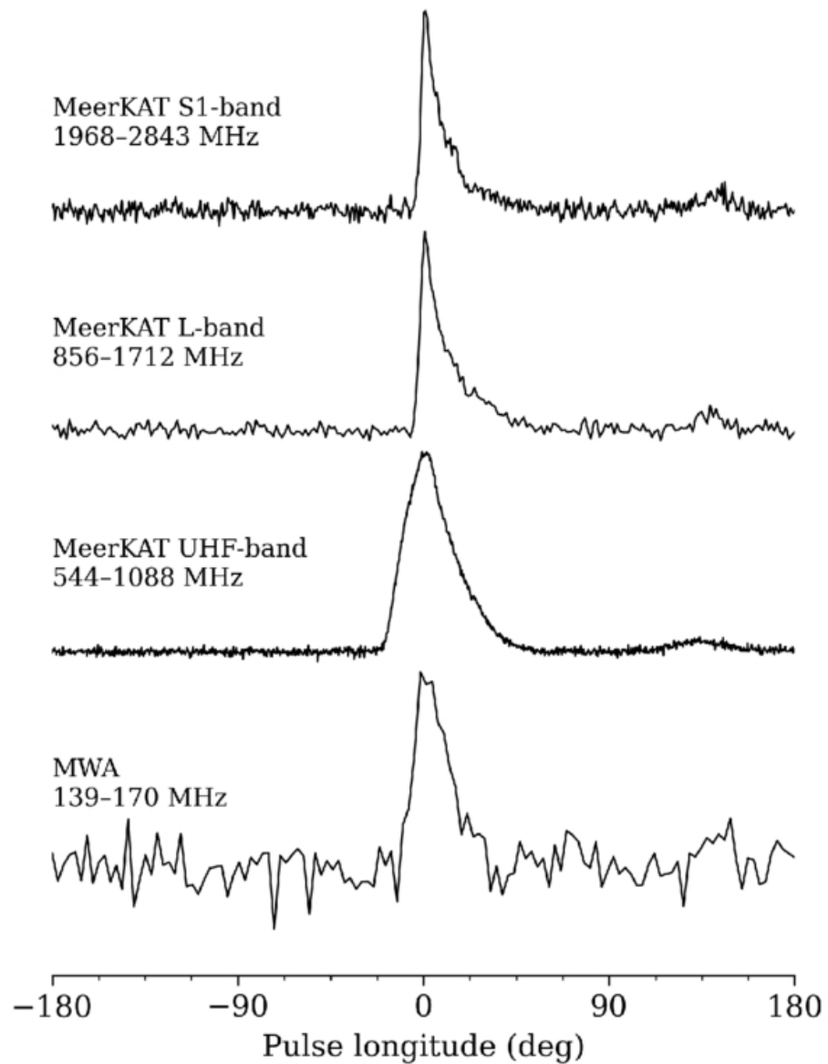
Figure 4. from Chia Min Tan et al 2026 Astrophys. J. Lett. 1006 doi:10.3847/2041-8213/ae7de5 https://dx.doi.org/10.3847/2041-8213/ae7de5 © 2026. The Author(s). Published by the American Astronomical Society.
