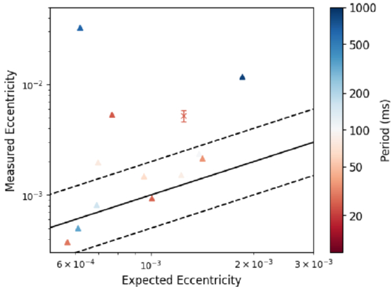
Figure 11. from Chia Min Tan et al 2026 Astrophys. J. Lett. 1006 doi:10.3847/2041-8213/ae7de5 https://dx.doi.org/10.3847/2041-8213/ae7de5 © 2026. The Author(s). Published by the American Astronomical Society.
