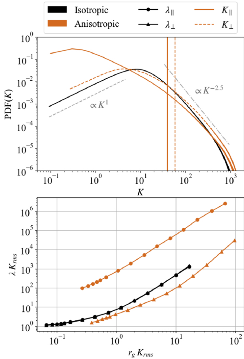
Figure 4. from Daniela Maci et al 2026 Astrophys. J. Lett. 1005 doi:10.3847/2041-8213/ae7d2b https://dx.doi.org/10.3847/2041-8213/ae7d2b © 2026. The Author(s). Published by the American Astronomical Society.
