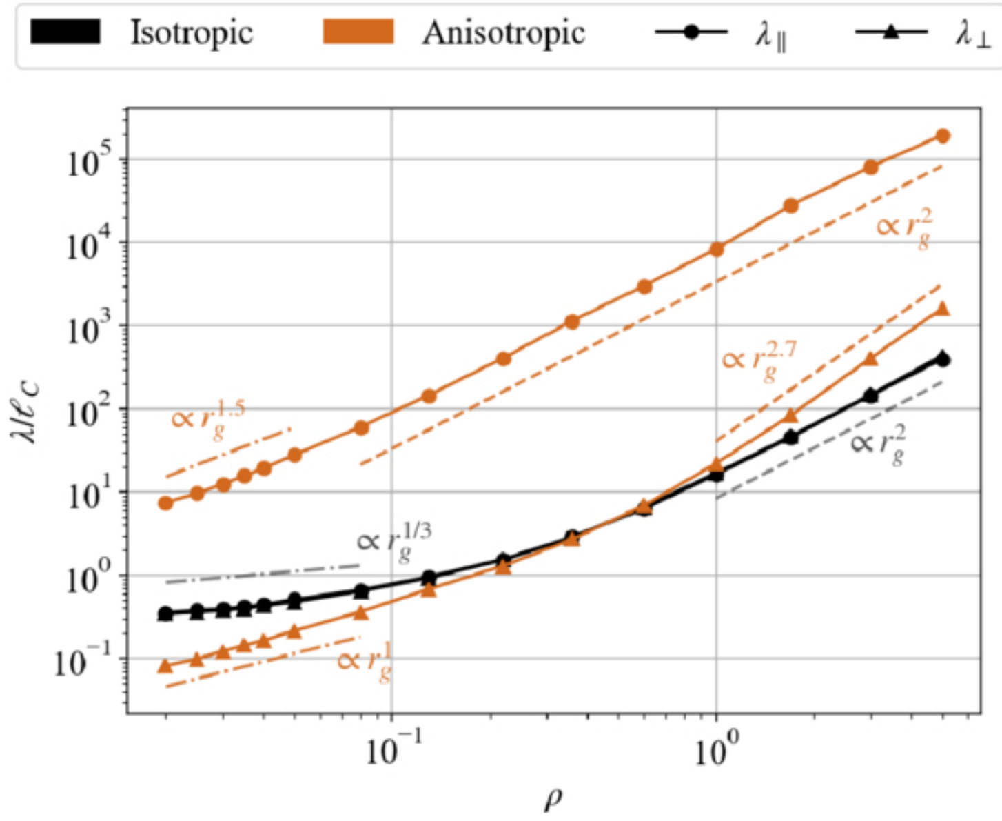
Figure 3. from Daniela Maci et al 2026 Astrophys. J. Lett. 1005 doi:10.3847/2041-8213/ae7d2b https://dx.doi.org/10.3847/2041-8213/ae7d2b © 2026. The Author(s). Published by the American Astronomical Society.
