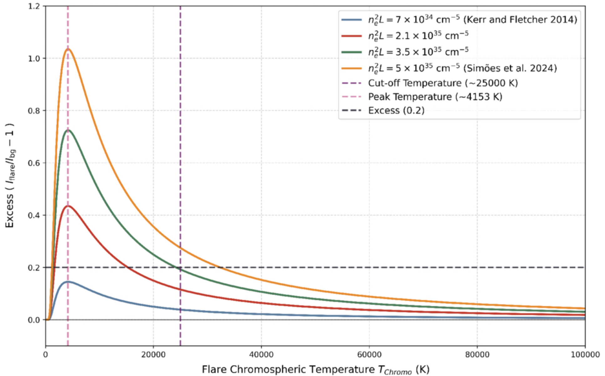
Figure 3. from Yingjie Cai et al 2026 Astrophys. J. Lett. 1005 doi:10.3847/2041-8213/ae7d19 https://dx.doi.org/10.3847/2041-8213/ae7d19 © 2026. The Author(s). Published by the American Astronomical Society.
