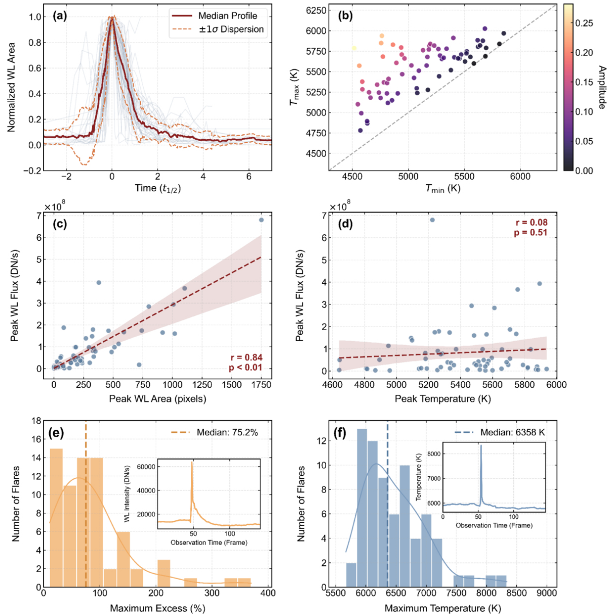
Figure 2. from Yingjie Cai et al 2026 Astrophys. J. Lett. 1005 doi:10.3847/2041-8213/ae7d19 https://dx.doi.org/10.3847/2041-8213/ae7d19 © 2026. The Author(s). Published by the American Astronomical Society.
