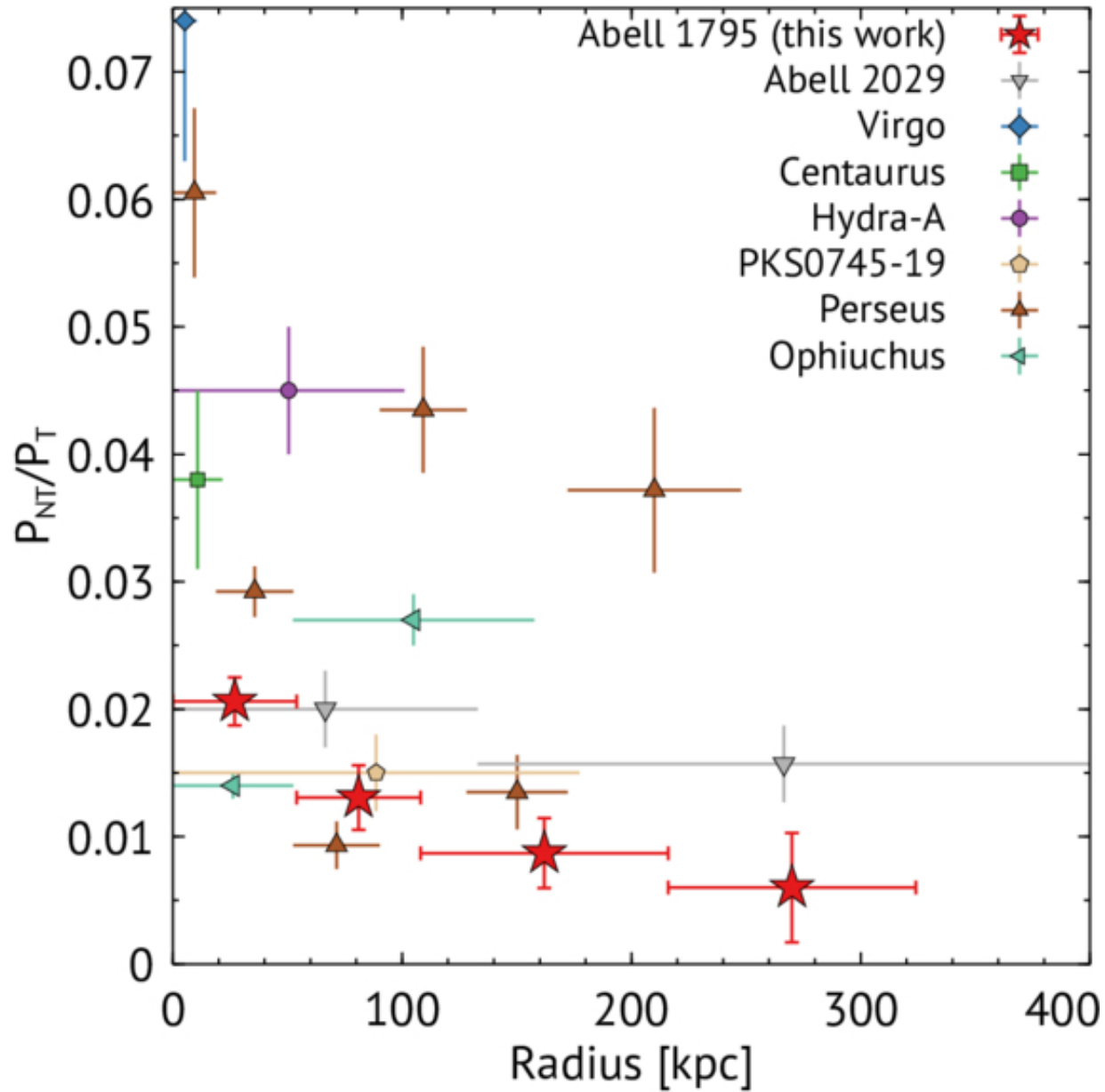
Figure 6. from Arnab Sarkar et al 2026 Astrophys. J. Lett. 1005 doi:10.3847/2041-8213/ae7d12 https://dx.doi.org/10.3847/2041-8213/ae7d12 © 2026. The Author(s). Published by the American Astronomical Society.
