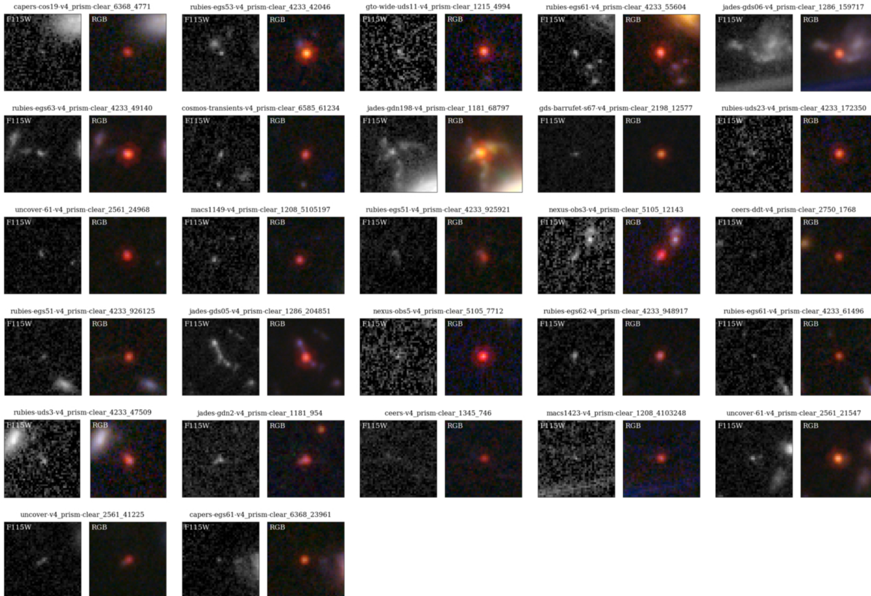
Figure 7. from Yoshihisa Asada et al 2026 Astrophys. J. Lett. 1005 doi:10.3847/2041-8213/ae7d0a https://dx.doi.org/10.3847/2041-8213/ae7d0a © 2026. The Author(s). Published by the American Astronomical Society.
