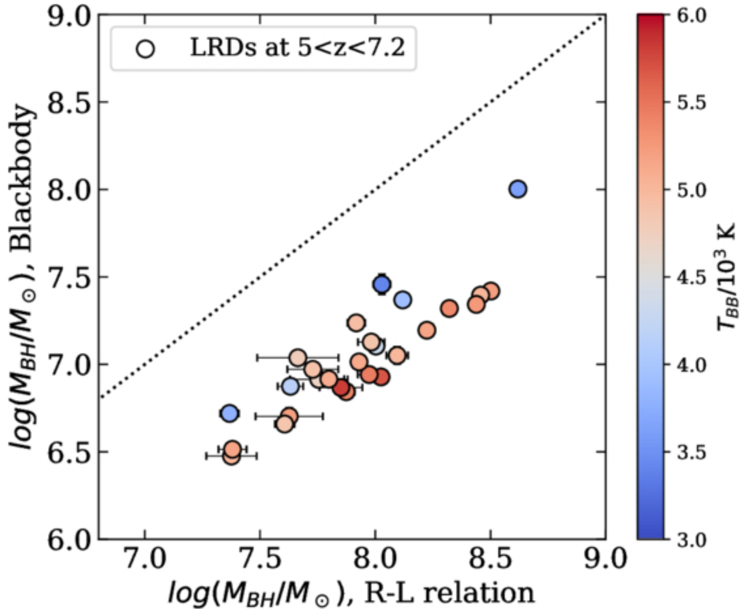
Figure 6. from Yoshihisa Asada et al 2026 Astrophys. J. Lett. 1005 doi:10.3847/2041-8213/ae7d0a https://dx.doi.org/10.3847/2041-8213/ae7d0a © 2026. The Author(s). Published by the American Astronomical Society.
