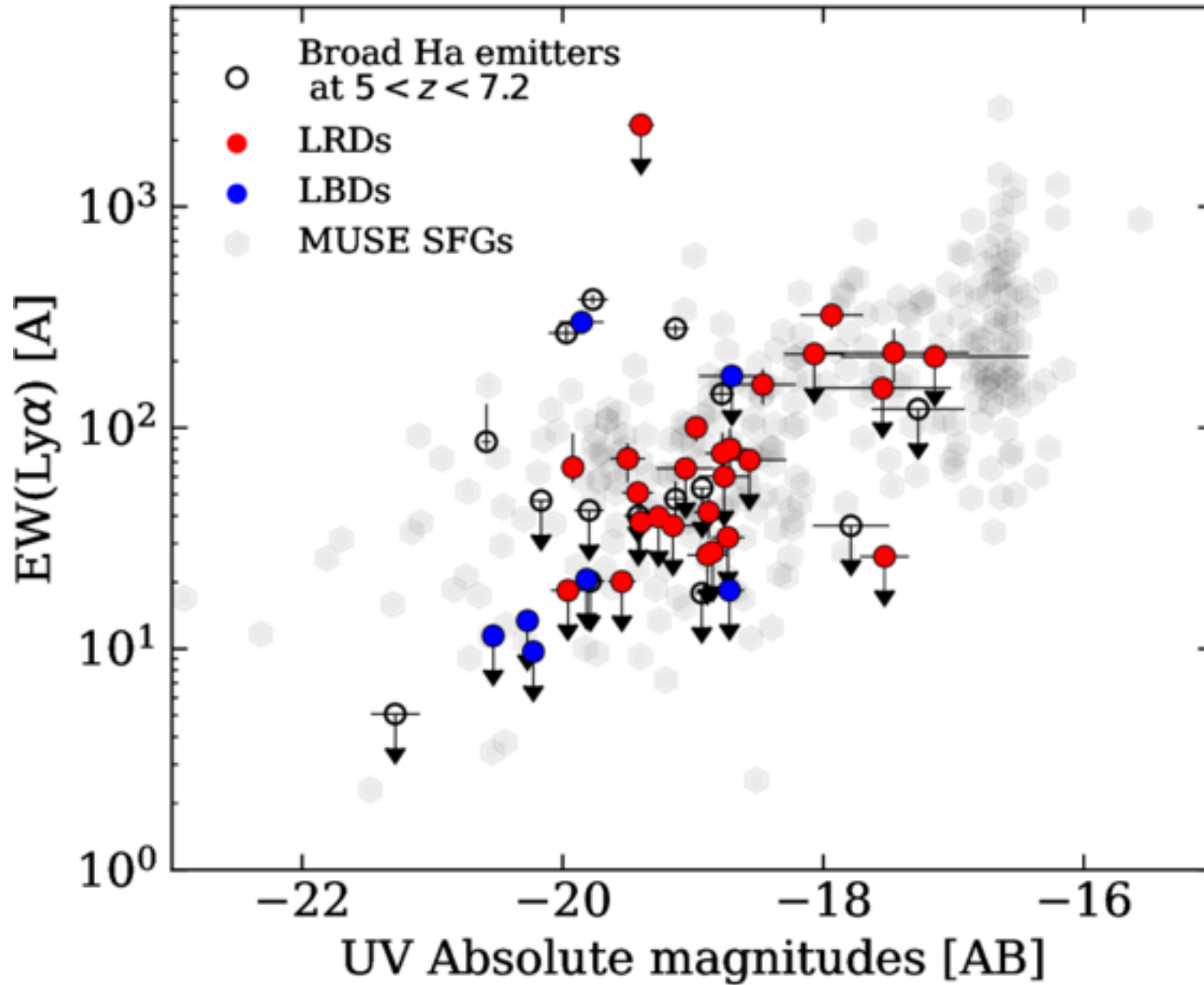
Figure 4. from Yoshihisa Asada et al 2026 Astrophys. J. Lett. 1005 doi:10.3847/2041-8213/ae7d0a https://dx.doi.org/10.3847/2041-8213/ae7d0a © 2026. The Author(s). Published by the American Astronomical Society.
