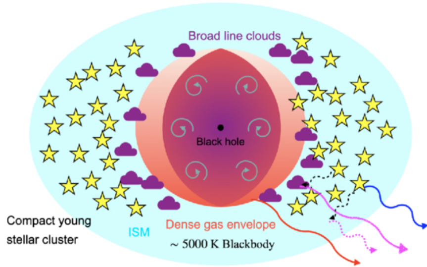
(a) Blackbody envelope model
