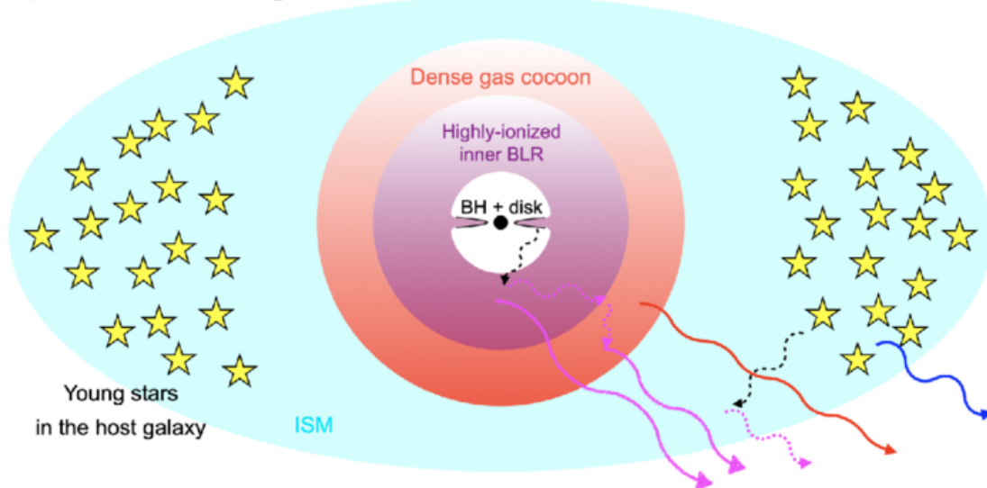
(b) Cocoon envelope model
