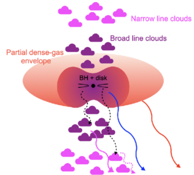
(c) Non-spherical envelope model
