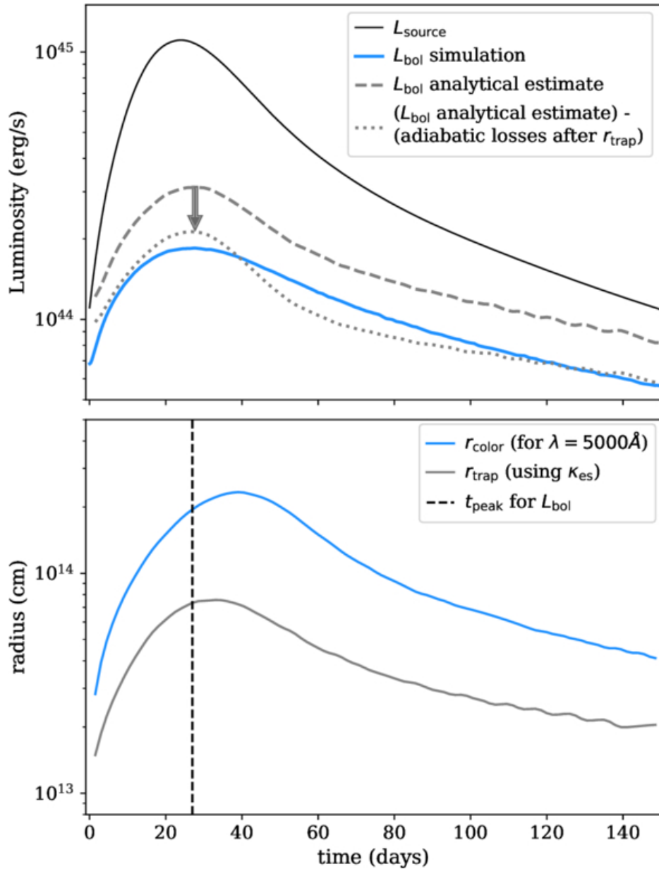
Figure 5. from Brenna Mockler et al 2026 Astrophys. J. Lett. 1005 doi:10.3847/2041-8213/ae7c6b https://dx.doi.org/10.3847/2041-8213/ae7c6b © 2026. The Author(s). Published by the American Astronomical Society.
