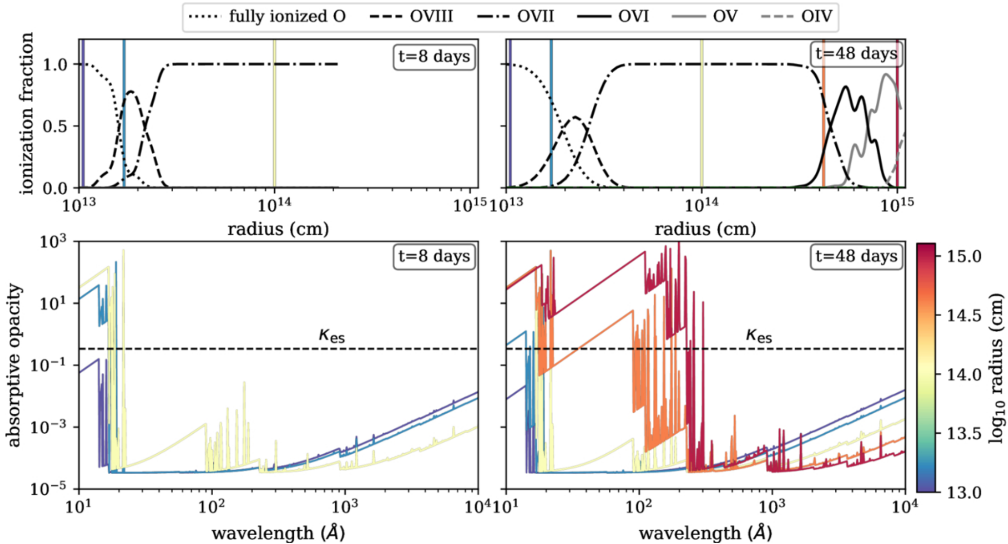
Figure 4. from Brenna Mockler et al 2026 Astrophys. J. Lett. 1005 doi:10.3847/2041-8213/ae7c6b https://dx.doi.org/10.3847/2041-8213/ae7c6b © 2026. The Author(s). Published by the American Astronomical Society.
