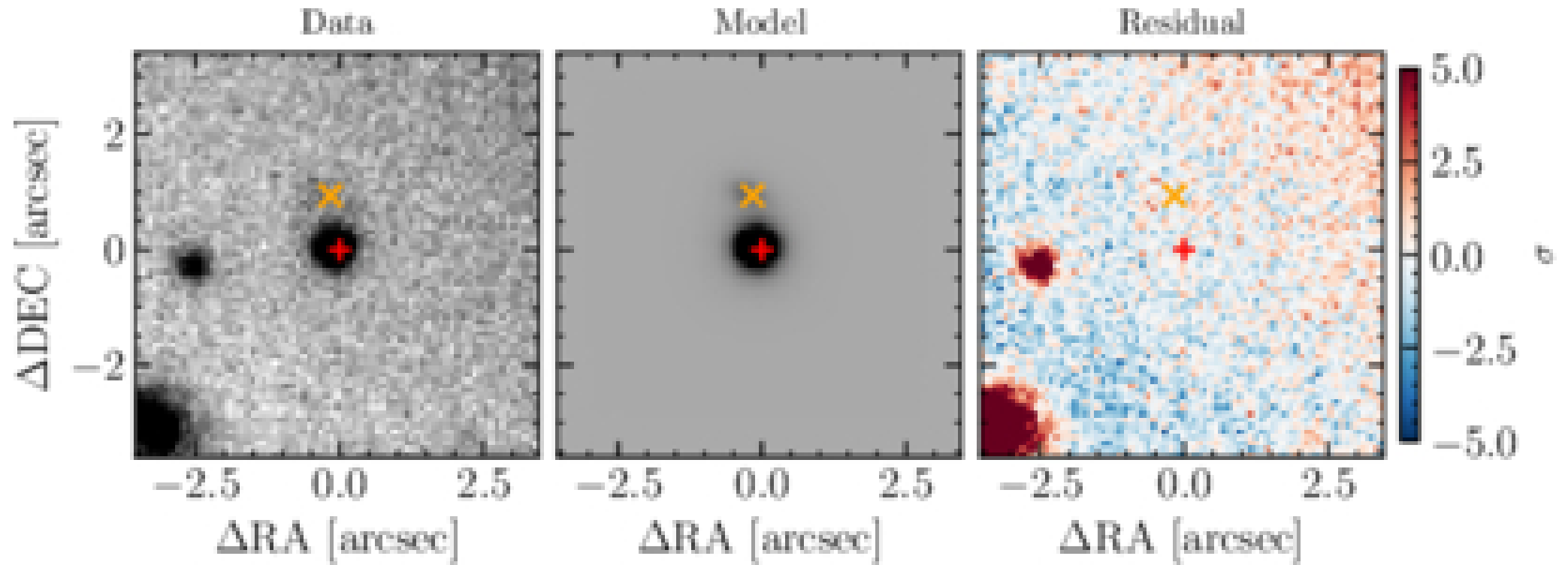
Figure 8. from Alberto Torralba et al 2026 Astrophys. J. Lett. 1005 doi:10.3847/2041-8213/ae7bfd https://dx.doi.org/10.3847/2041-8213/ae7bfd © 2026. The Author(s). Published by the American Astronomical Society.
