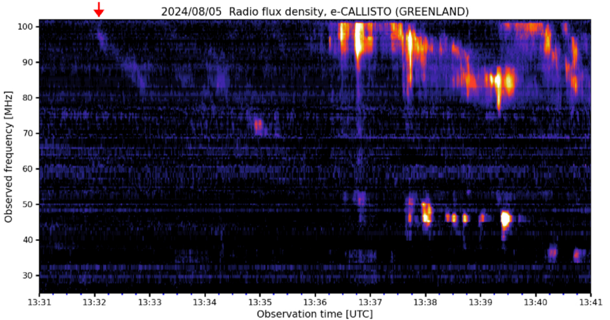
Figure 3. from R. Ramesh et al 2026 Astrophys. J. Lett. 1005 doi:10.3847/2041-8213/ae7bf0 https://dx.doi.org/10.3847/2041-8213/ae7bf0 © 2026. The Author(s). Published by the American Astronomical Society.
