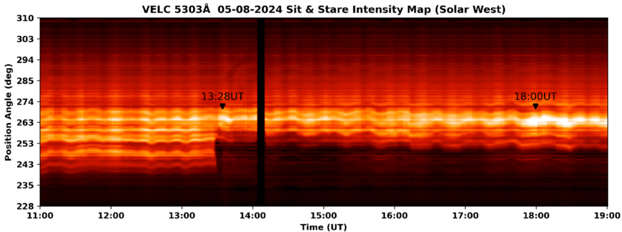
Figure 2. from R. Ramesh et al 2026 Astrophys. J. Lett. 1005 doi:10.3847/2041-8213/ae7bf0 https://dx.doi.org/10.3847/2041-8213/ae7bf0 © 2026. The Author(s). Published by the American Astronomical Society.
