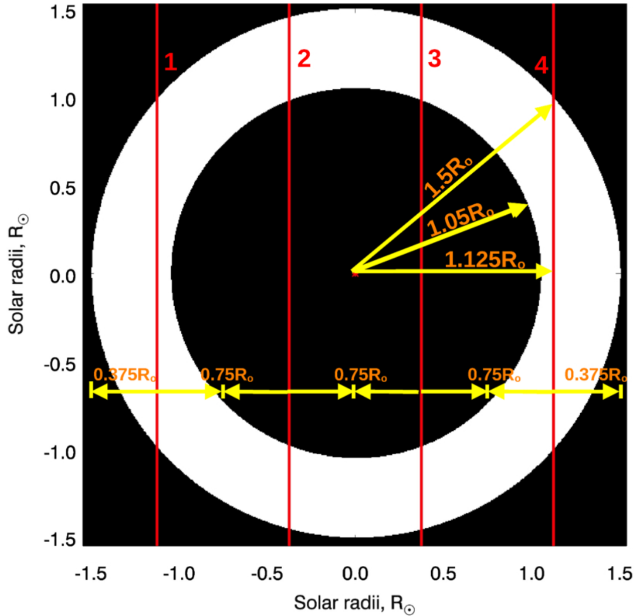
Figure 1. from R. Ramesh et al 2026 Astrophys. J. Lett. 1005 doi:10.3847/2041-8213/ae7bf0 https://dx.doi.org/10.3847/2041-8213/ae7bf0 © 2026. The Author(s). Published by the American Astronomical Society.
