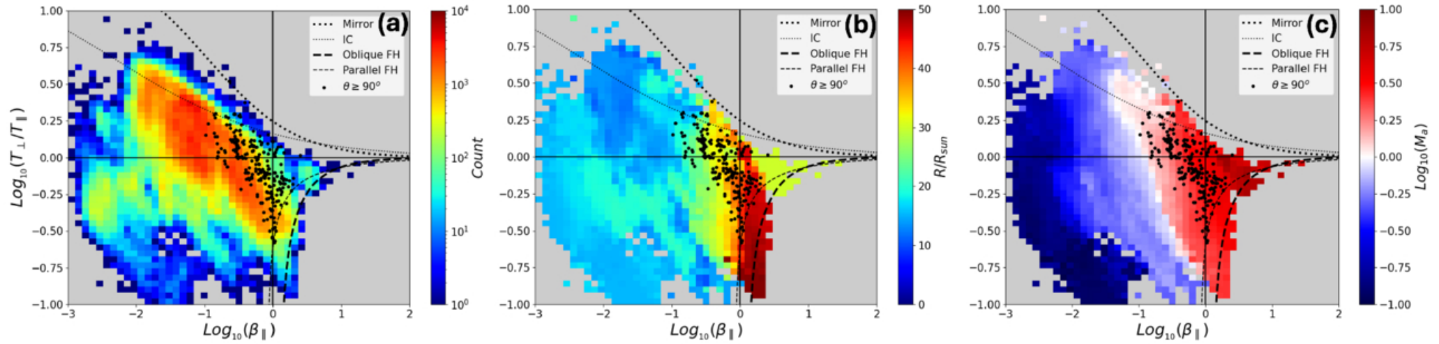
Figure 1. from Dominic Payne et al 2026 Astrophys. J. Lett. 1005 doi:10.3847/2041-8213/ae7bef https://dx.doi.org/10.3847/2041-8213/ae7bef © 2026. The Author(s). Published by the American Astronomical Society.
