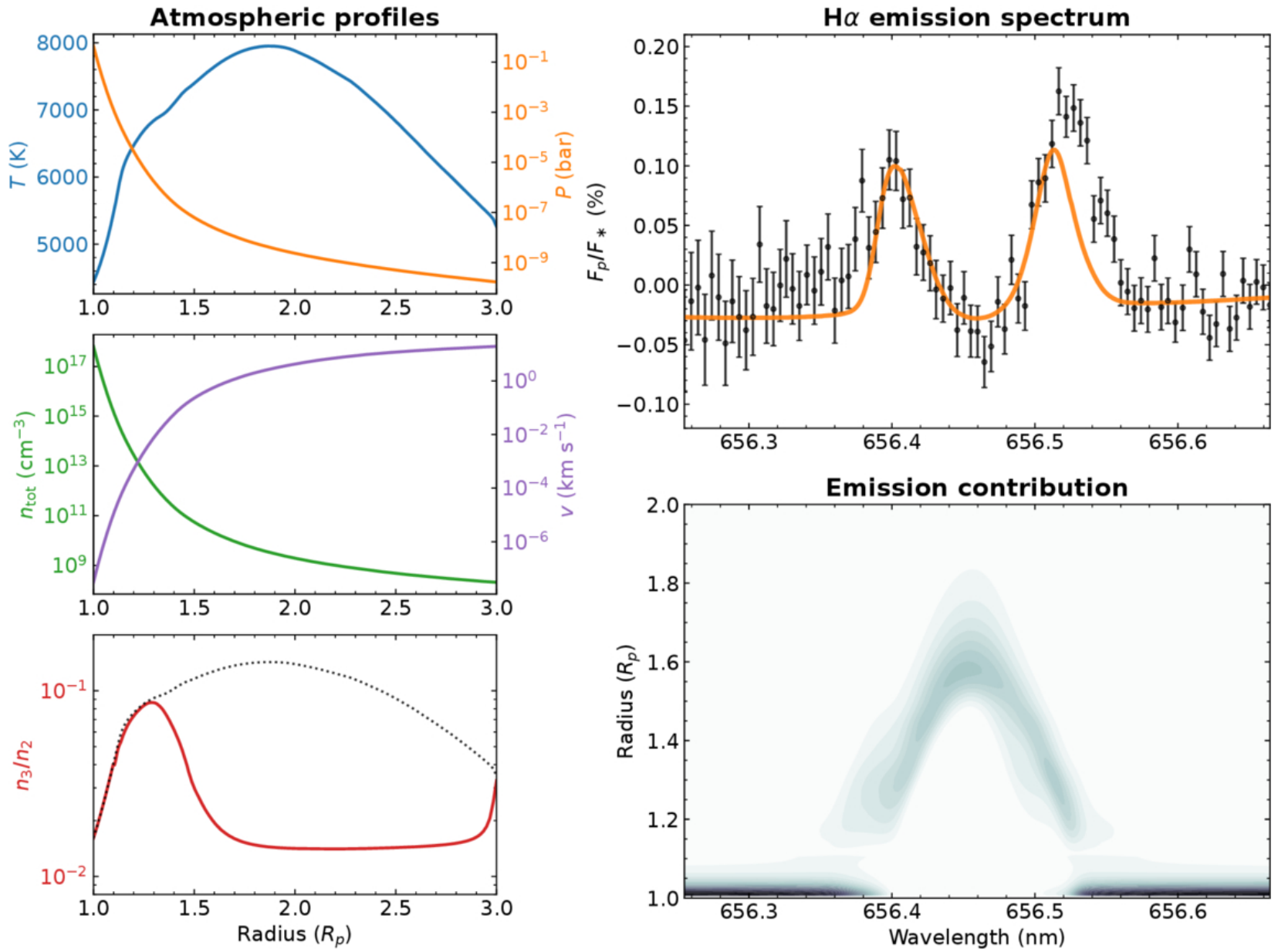
Figure 2. from Yapeng Zhang et al 2026 Astrophys. J. Lett. 1005 doi:10.3847/2041-8213/ae7be6 https://dx.doi.org/10.3847/2041-8213/ae7be6 © 2026. The Author(s). Published by the American Astronomical Society.
