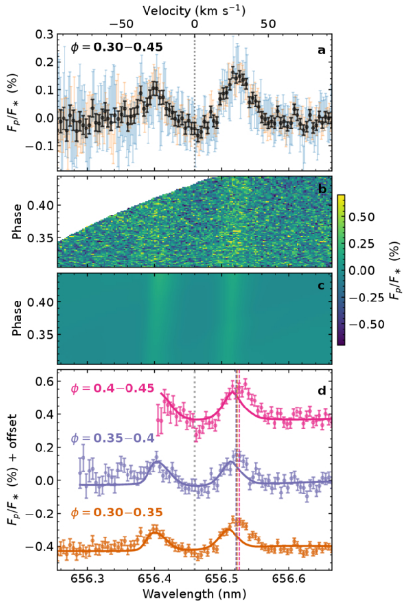
Figure 1. from Yapeng Zhang et al 2026 Astrophys. J. Lett. 1005 doi:10.3847/2041-8213/ae7be6 https://dx.doi.org/10.3847/2041-8213/ae7be6 © 2026. The Author(s). Published by the American Astronomical Society.
