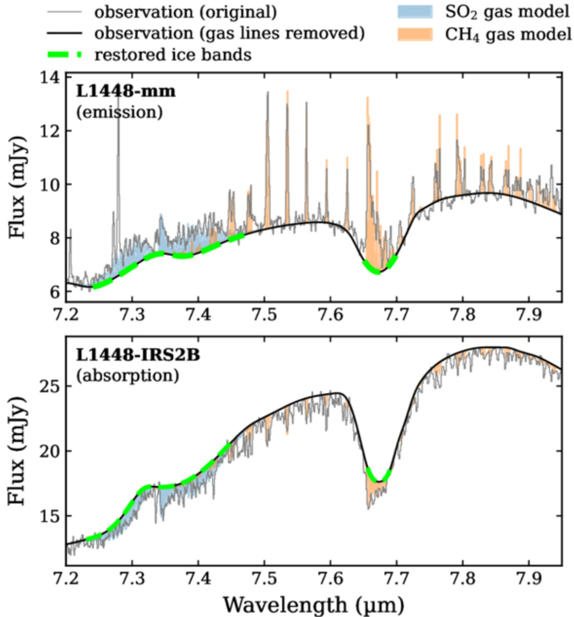
Figure 5. from Yuan Chen et al 2026 Astrophys. J. Lett. 1005 doi:10.3847/2041-8213/ae7a70 https://dx.doi.org/10.3847/2041-8213/ae7a70 © 2026. The Author(s). Published by the American Astronomical Society.
