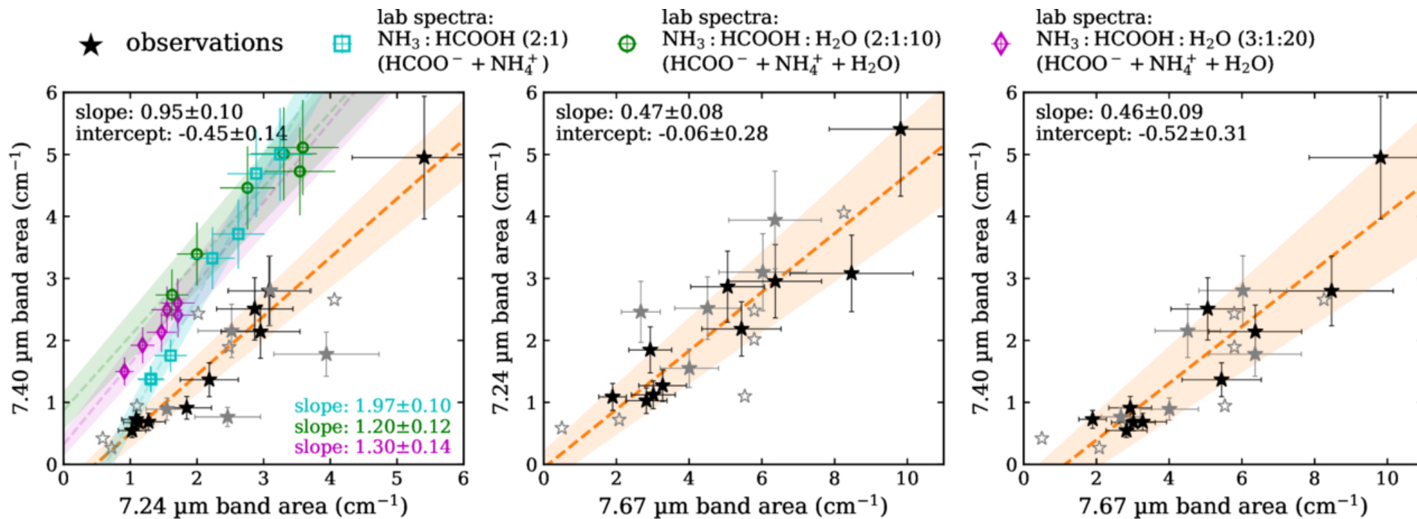
Figure 3. from Yuan Chen et al 2026 Astrophys. J. Lett. 1005 doi:10.3847/2041-8213/ae7a70 https://dx.doi.org/10.3847/2041-8213/ae7a70 © 2026. The Author(s). Published by the American Astronomical Society.
