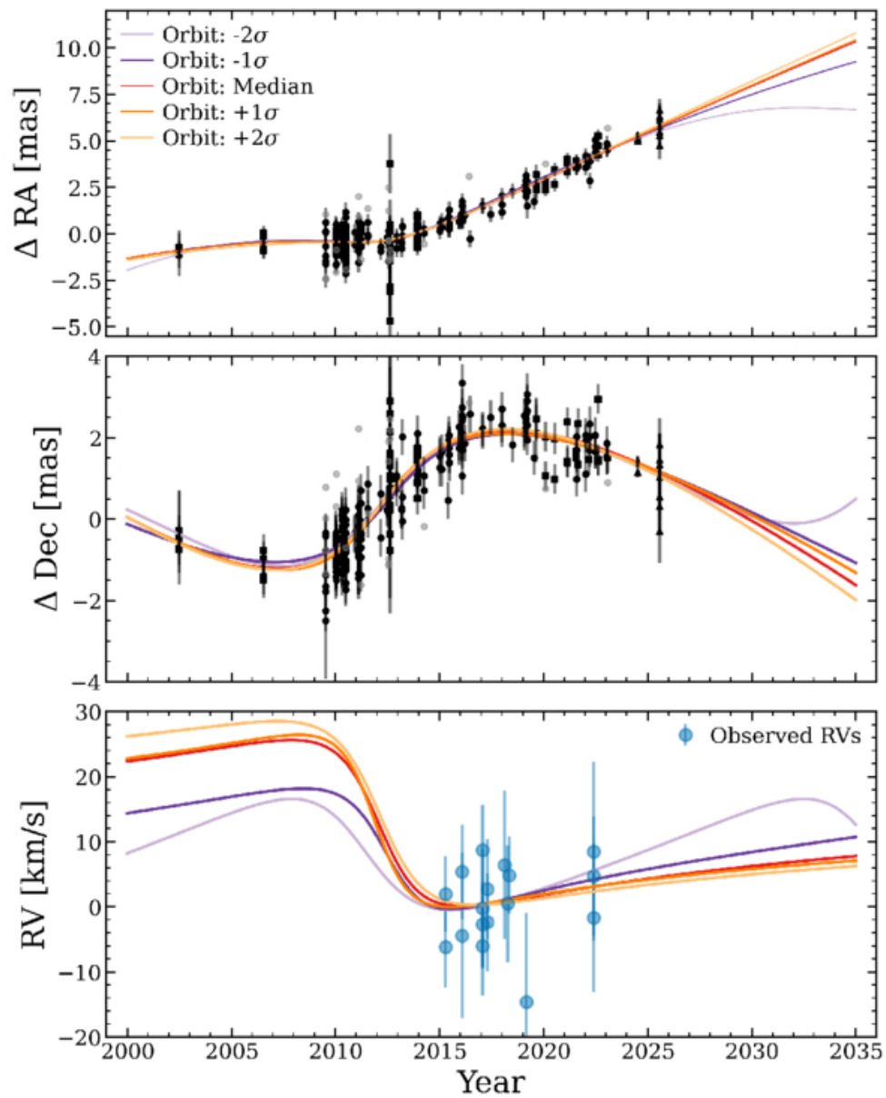
Figure 9. from Matthew Whitaker et al 2026 Astrophys. J. Lett. 1006 doi:10.3847/2041-8213/ae7a5c https://dx.doi.org/10.3847/2041-8213/ae7a5c © 2026. The Author(s). Published by the American Astronomical Society.
