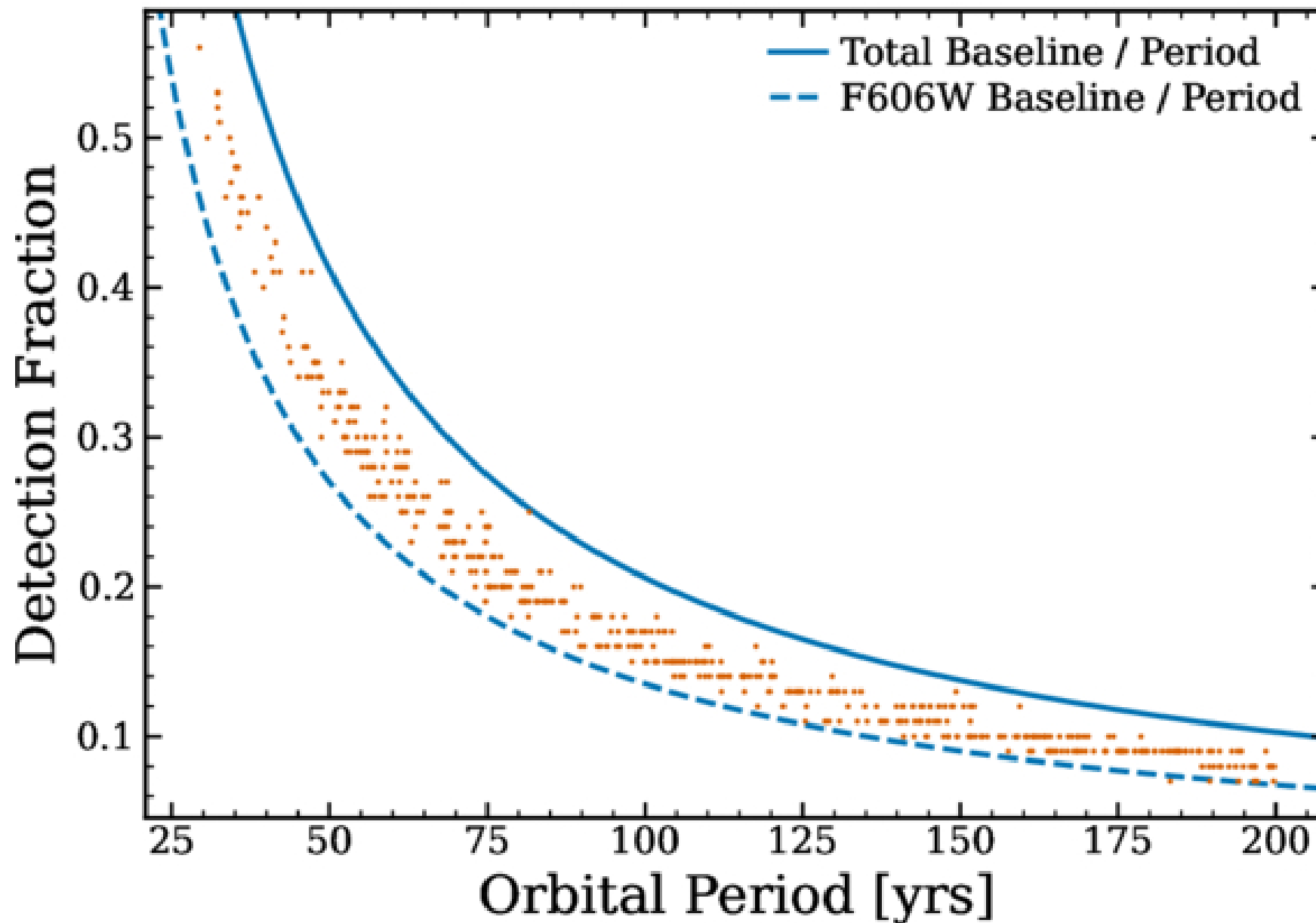
Figure 7. from Matthew Whitaker et al 2026 Astrophys. J. Lett. 1006 doi:10.3847/2041-8213/ae7a5c https://dx.doi.org/10.3847/2041-8213/ae7a5c © 2026. The Author(s). Published by the American Astronomical Society.
