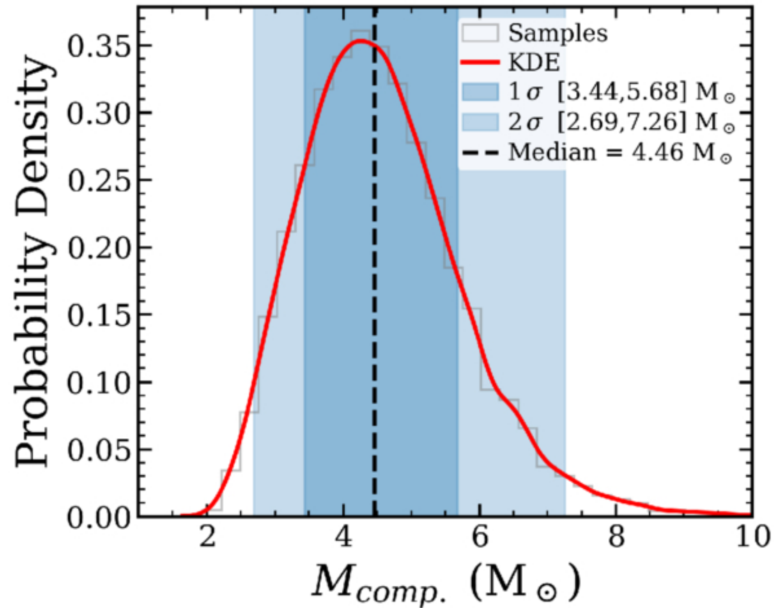
Figure 6. from Matthew Whitaker et al 2026 Astrophys. J. Lett. 1006 doi:10.3847/2041-8213/ae7a5c https://dx.doi.org/10.3847/2041-8213/ae7a5c © 2026. The Author(s). Published by the American Astronomical Society.
