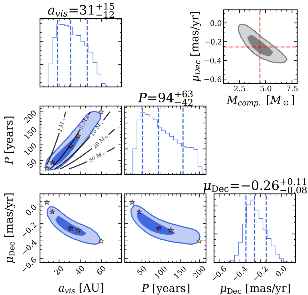
Figure 5. from Matthew Whitaker et al 2026 Astrophys. J. Lett. 1006 doi:10.3847/2041-8213/ae7a5c https://dx.doi.org/10.3847/2041-8213/ae7a5c © 2026. The Author(s). Published by the American Astronomical Society.
