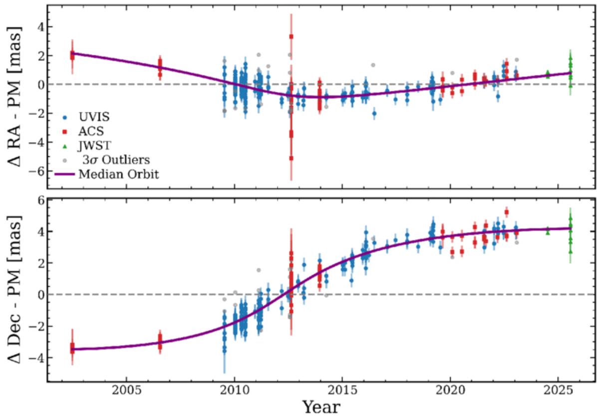
Figure 4. from Matthew Whitaker et al 2026 Astrophys. J. Lett. 1006 doi:10.3847/2041-8213/ae7a5c https://dx.doi.org/10.3847/2041-8213/ae7a5c © 2026. The Author(s). Published by the American Astronomical Society.
