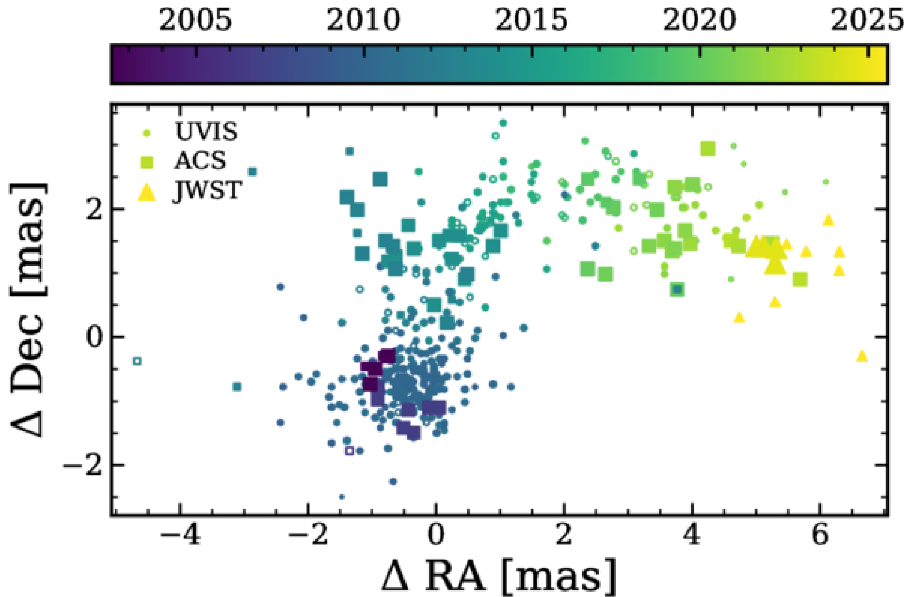
Figure 3. from Matthew Whitaker et al 2026 Astrophys. J. Lett. 1006 doi:10.3847/2041-8213/ae7a5c https://dx.doi.org/10.3847/2041-8213/ae7a5c © 2026. The Author(s). Published by the American Astronomical Society.
