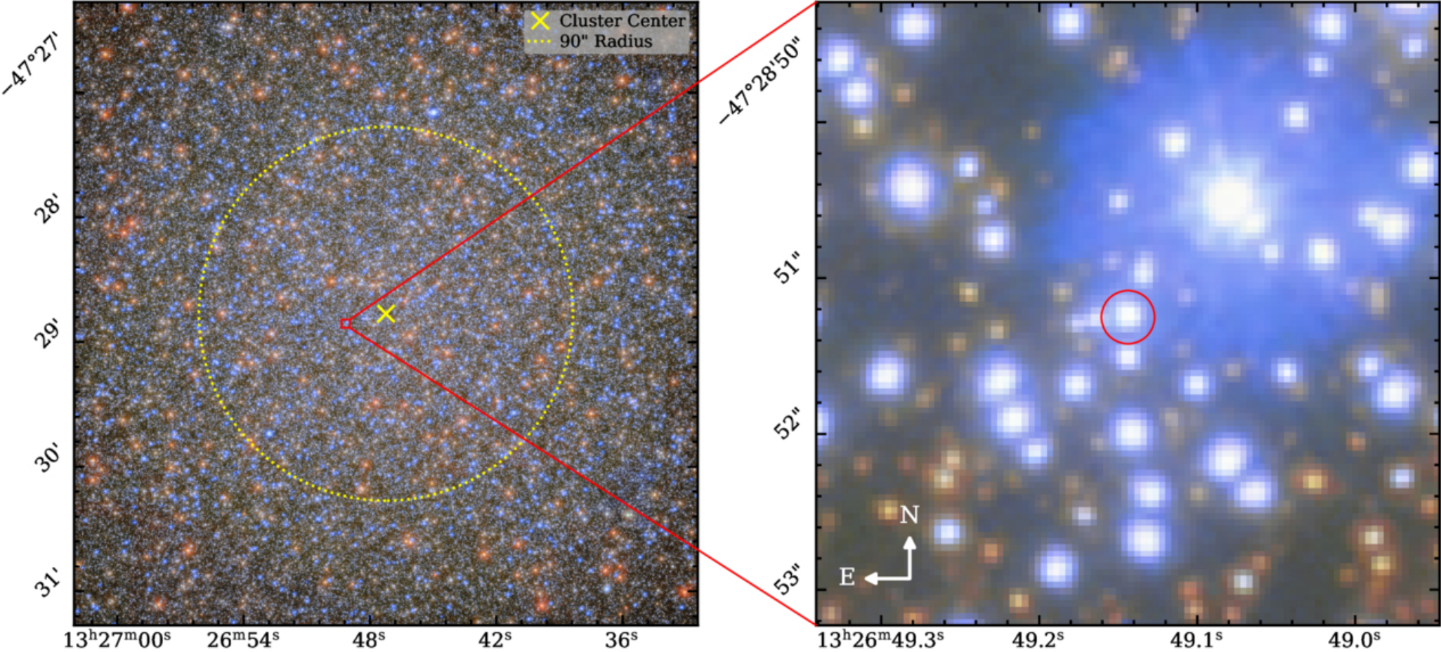
Figure 1. from Matthew Whitaker et al 2026 Astrophys. J. Lett. 1006 doi:10.3847/2041-8213/ae7a5c https://dx.doi.org/10.3847/2041-8213/ae7a5c © 2026. The Author(s). Published by the American Astronomical Society.
