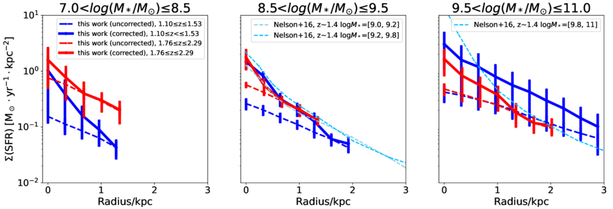
Figure 5. from Pengfei Ren et al 2026 Astrophys. J. Lett. 1005 doi:10.3847/2041-8213/ae7a35 https://dx.doi.org/10.3847/2041-8213/ae7a35 © 2026. The Author(s). Published by the American Astronomical Society.
