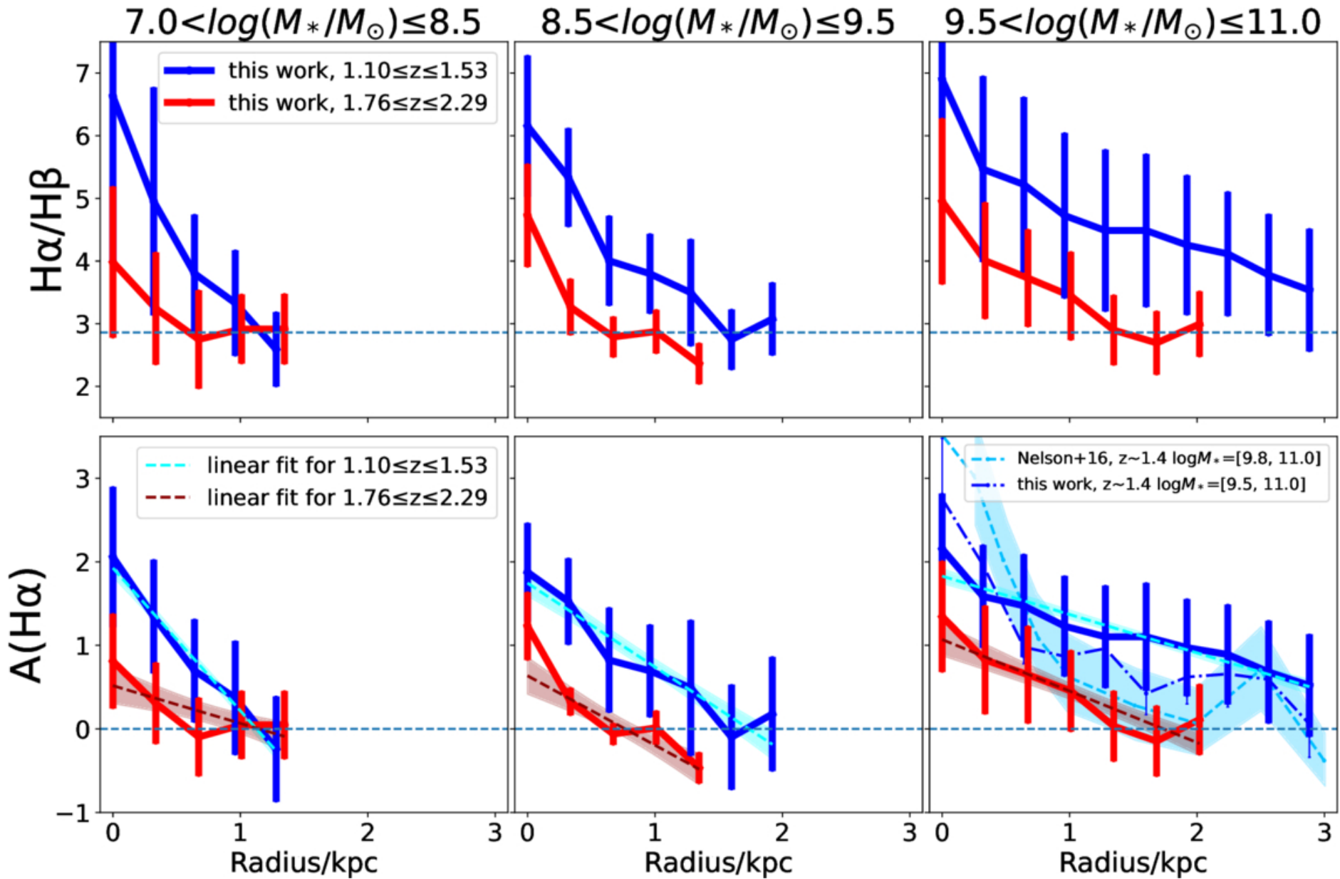
Figure 4. from Pengfei Ren et al 2026 Astrophys. J. Lett. 1005 doi:10.3847/2041-8213/ae7a35 https://dx.doi.org/10.3847/2041-8213/ae7a35 © 2026. The Author(s). Published by the American Astronomical Society.
