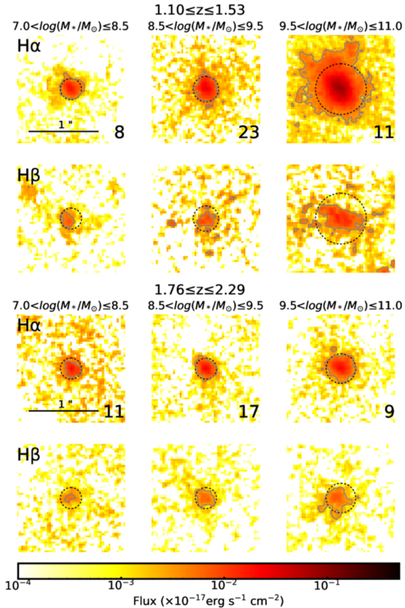
Figure 3. from Pengfei Ren et al 2026 Astrophys. J. Lett. 1005 doi:10.3847/2041-8213/ae7a35 https://dx.doi.org/10.3847/2041-8213/ae7a35 © 2026. The Author(s). Published by the American Astronomical Society.
