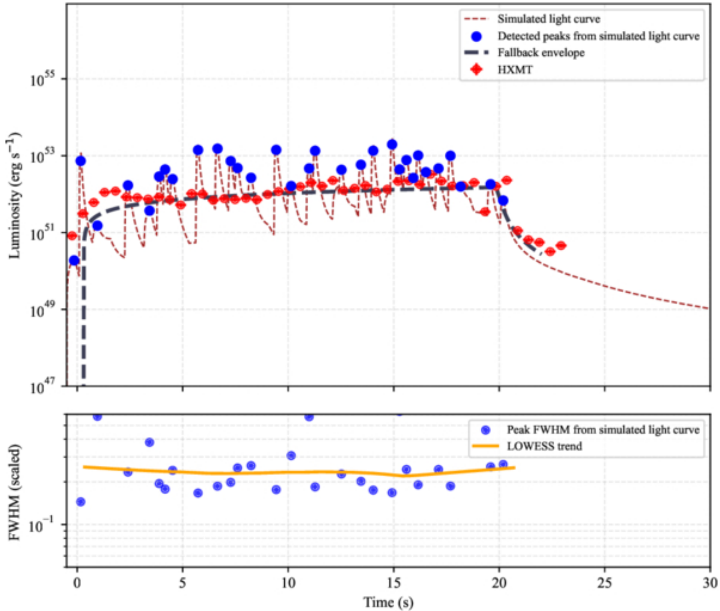
Figure 4. from Chen-Wei Wang et al 2026 Astrophys. J. Lett. 1004 doi:10.3847/2041-8213/ae7970 https://dx.doi.org/10.3847/2041-8213/ae7970 © 2026. The Author(s). Published by the American Astronomical Society.
