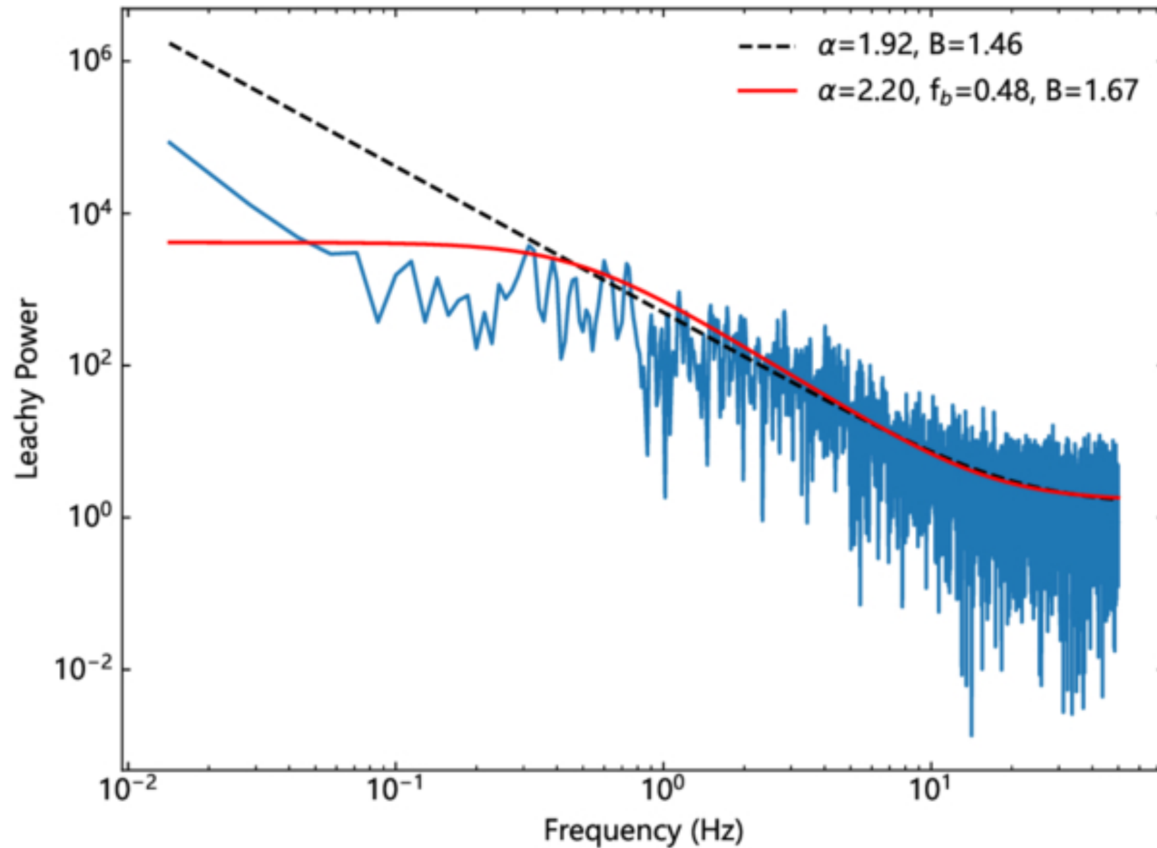
Figure 3. from Chen-Wei Wang et al 2026 Astrophys. J. Lett. 1004 doi:10.3847/2041-8213/ae7970 https://dx.doi.org/10.3847/2041-8213/ae7970 © 2026. The Author(s). Published by the American Astronomical Society.
