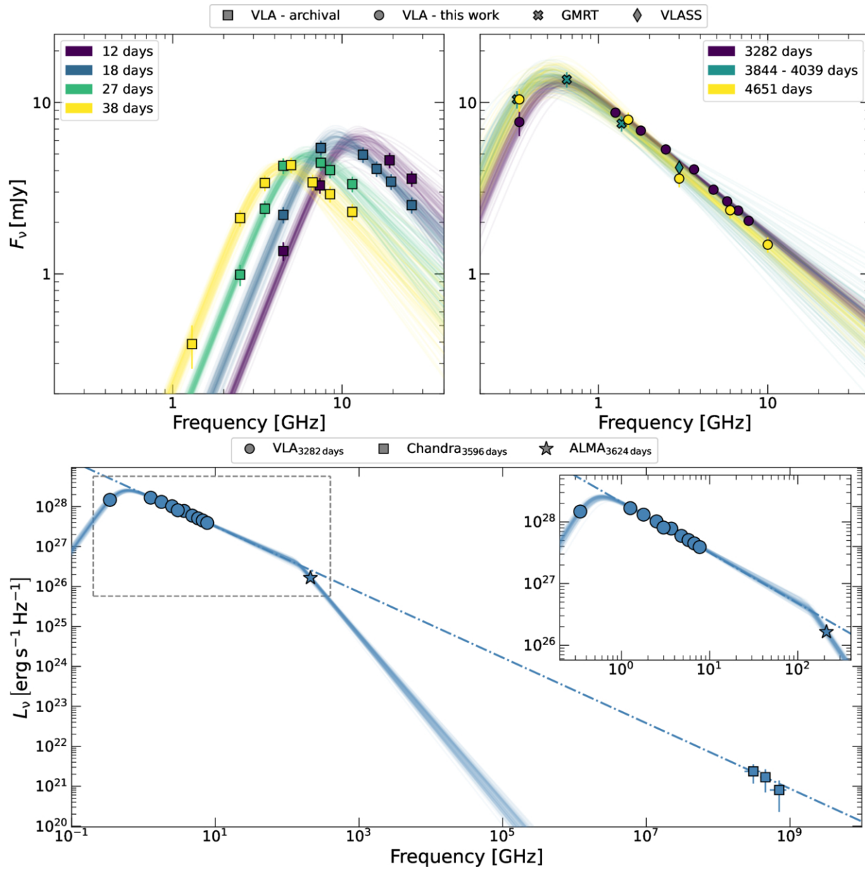
Figure 3. from Itai Sfaradi et al 2026 Astrophys. J. Lett. 1005 doi:10.3847/2041-8213/ae796d https://dx.doi.org/10.3847/2041-8213/ae796d © 2026. The Author(s). Published by the American Astronomical Society.
