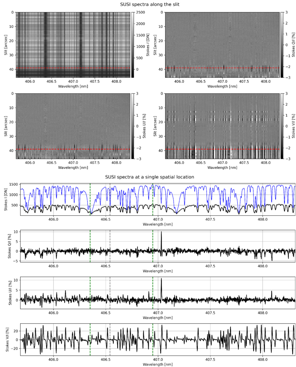
Figure 4. from Sami K. Solanki et al 2026 Astrophys. J. Lett. 1005 doi:10.3847/2041-8213/ae796b https://dx.doi.org/10.3847/2041-8213/ae796b © 2026. The Author(s). Published by the American Astronomical Society.
