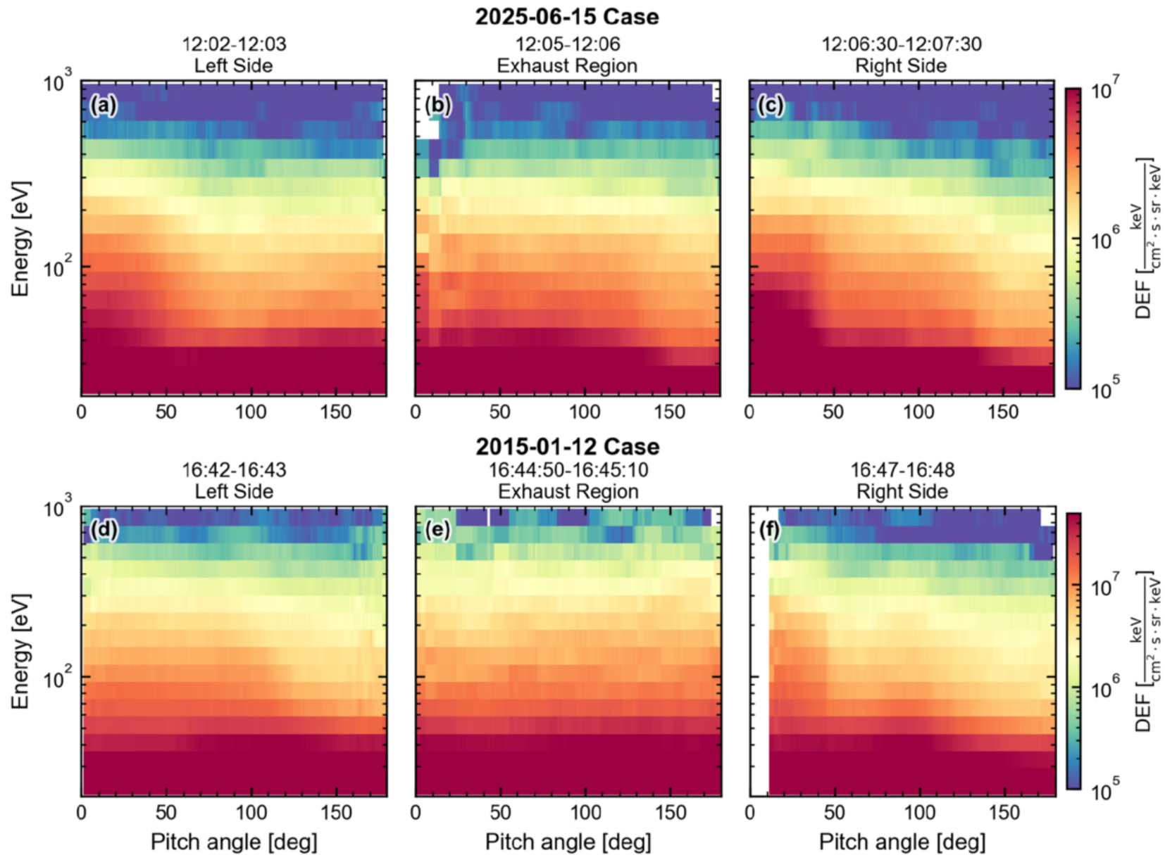
Figure B1. from Chi Zhang et al 2026 Astrophys. J. Lett. 1004 doi:10.3847/2041-8213/ae78dc https://dx.doi.org/10.3847/2041-8213/ae78dc © 2026. The Author(s). Published by the American Astronomical Society.
