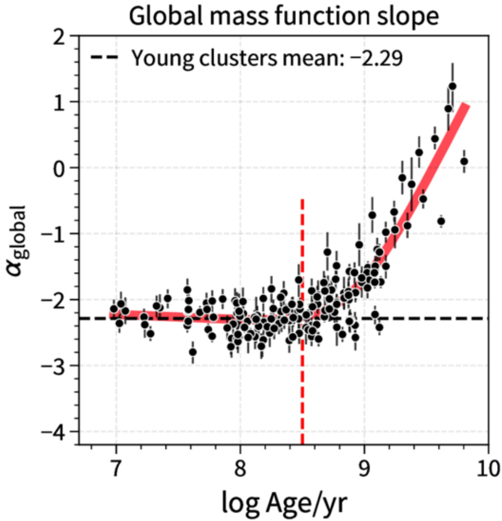
Figure 2. from Lu Li et al 2026 Astrophys. J. Lett. 1005 doi:10.3847/2041-8213/ae78cc https://dx.doi.org/10.3847/2041-8213/ae78cc © 2026. The Author(s). Published by the American Astronomical Society.
