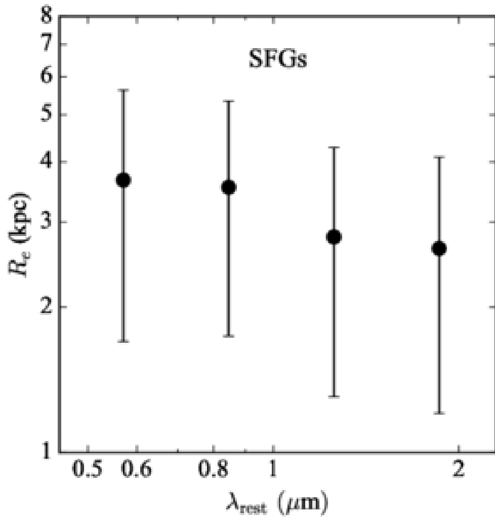
Figure A1. from Si-Yue Yu et al 2026 Astrophys. J. Lett. 1005 doi:10.3847/2041-8213/ae77f8 https://dx.doi.org/10.3847/2041-8213/ae77f8 © 2026. The Author(s). Published by the American Astronomical Society.
